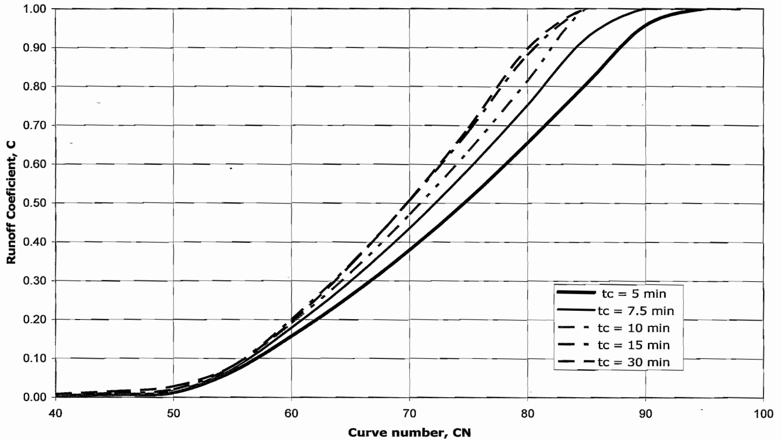
Figure 4. Runoff coefficients for 10-yr event below 1,640 ft (NRCS type 1 storm)
