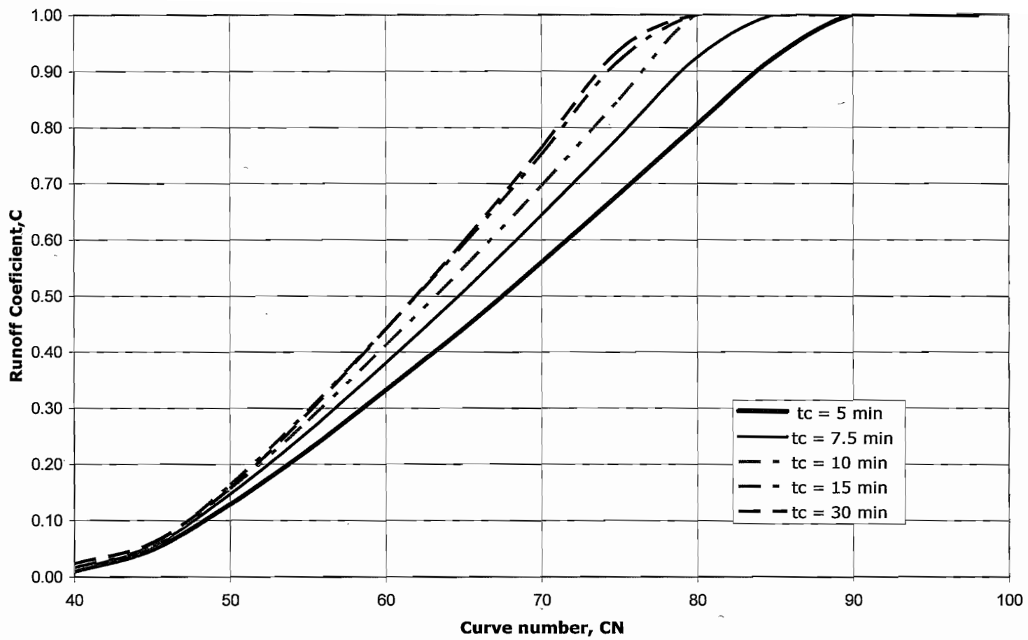
Figure 6. Runoff coefficients for 100-yr event below 1,640 ft (NRCS type 1 storm)
